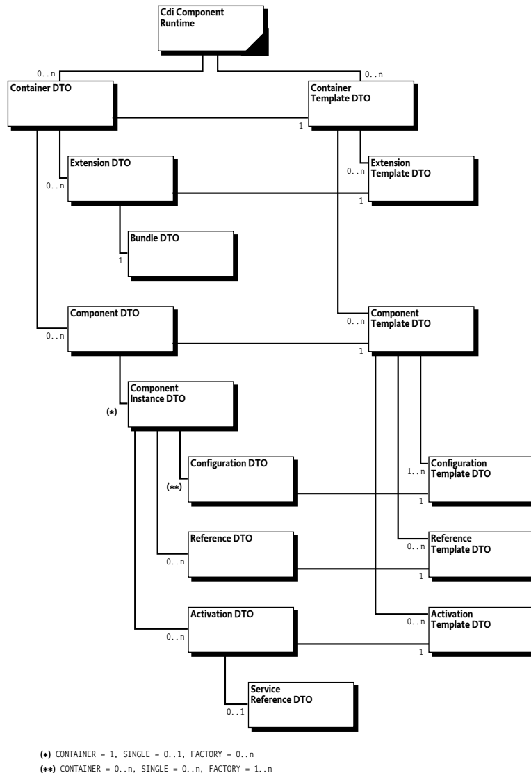
CDI Component Runtime DTOs
