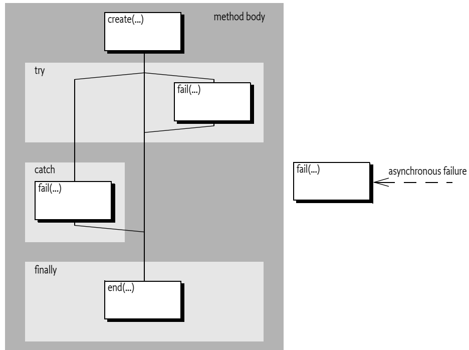
Flow through the Coordination template
