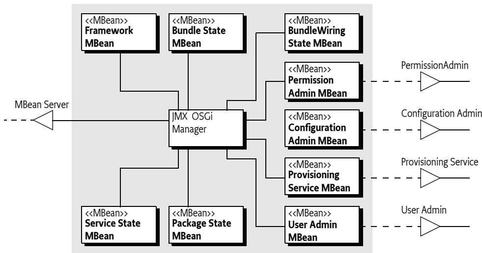
Figure 124.1 MBeans
