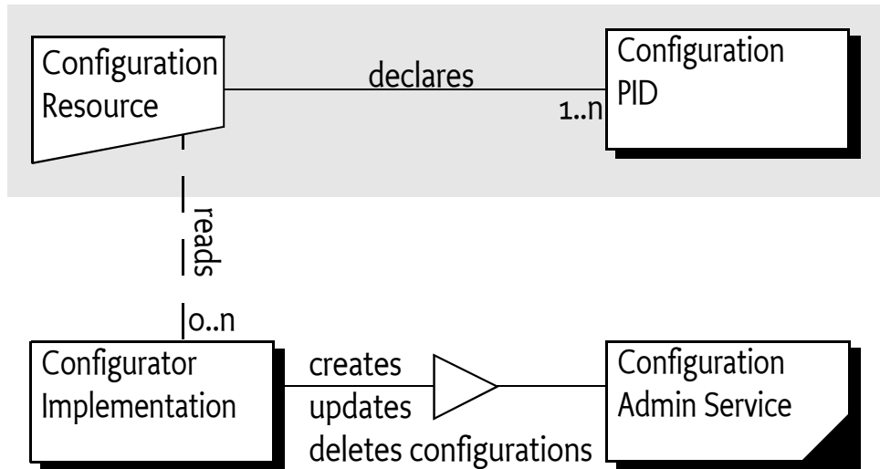
Configurator Entity Overview
