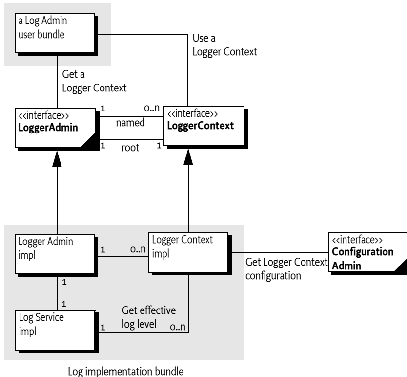
Log Admin Class Diagram org.osgi.service.log.admin package
